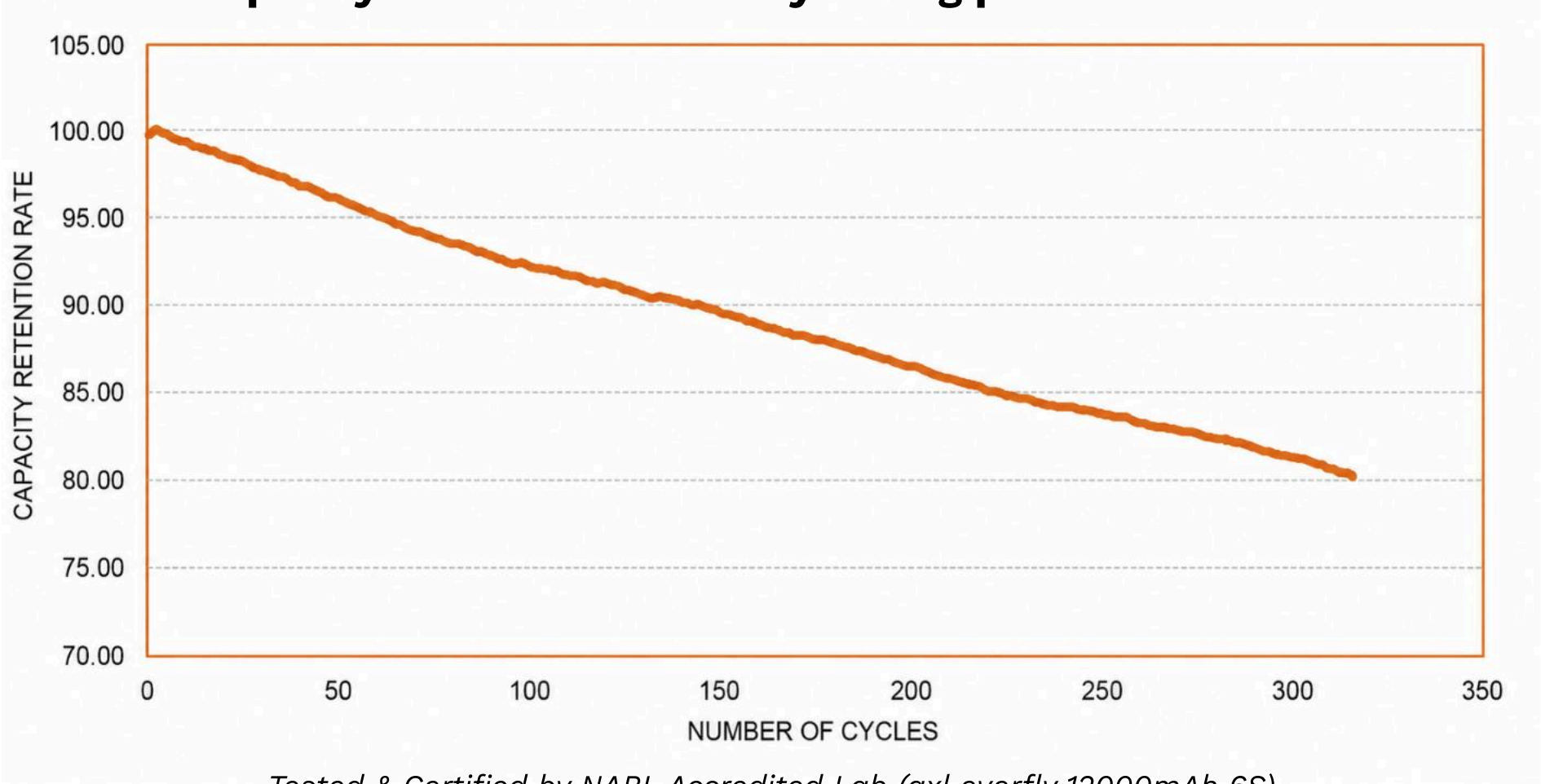
Capacity retention of battery during performance test
